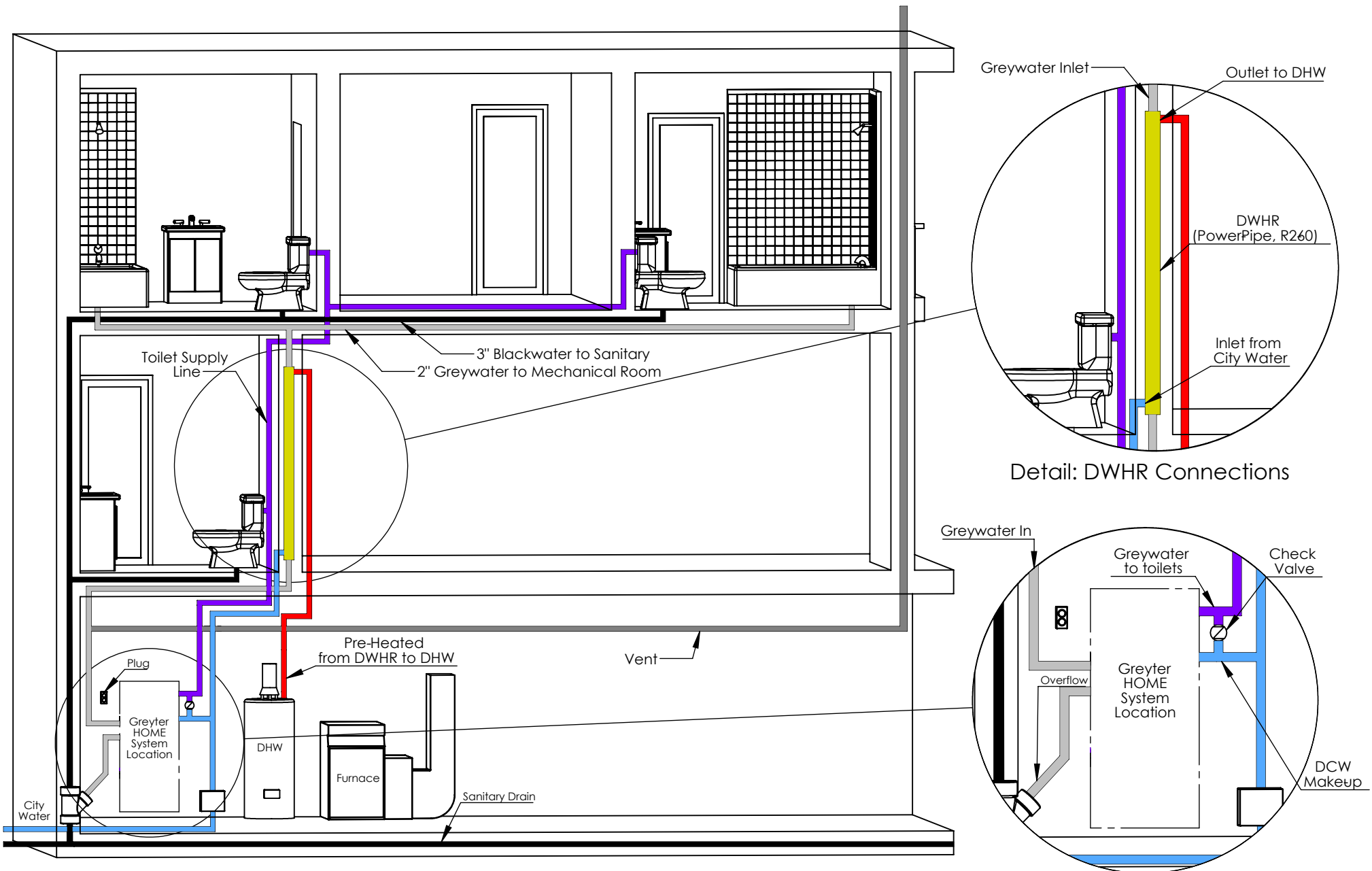
Detail: Greyter HOME System Connections
